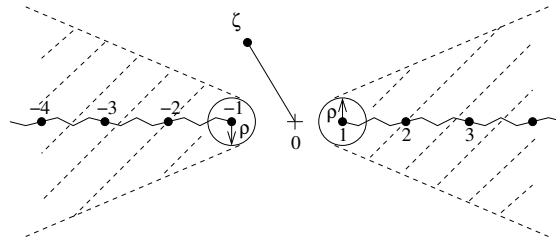
Fig. 3.1 The domain \mathcal{R}_\rho^{(0)} .
