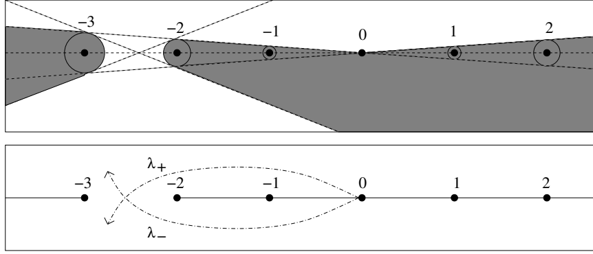
Fig. 4.7 Figure above, the domain \overset{\bullet}{\mathcal{R}}_\rho^{(+)_2, \pi} . Figure below, the domain \overset{\bullet}{\mathcal{R}}_\rho^{2, \pi} .
