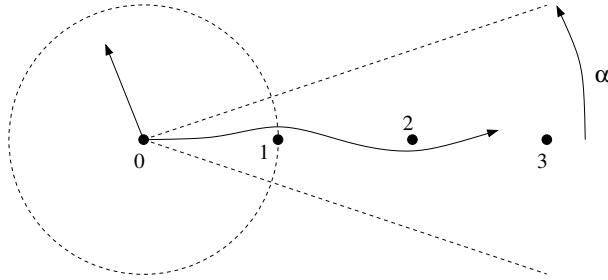
Fig. 4.10 Two paths belonging to \mathfrak{R}^{(\theta, \alpha)}(L) for \theta = 0 and L \geq 2 .
