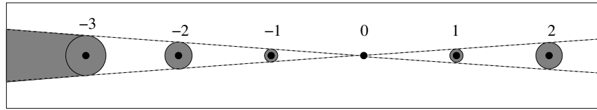
Fig. 4.4 The domain \mathring{\mathcal{R}}_\rho when \frac{1}{9} < \rho \leq \frac{1}{7} (the scale is not correct).
