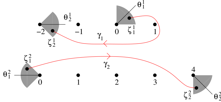
Fig. 7.11 The triple (\gamma_1, \theta_1^1, \theta_2^1) for the point \omega_1 = -2 , the triple (\gamma_2, \theta_1^2, \theta_2^2) for the point \omega_2 - \omega_1 = 4 , with \theta_2^2 = \theta_1^2 + \pi .
