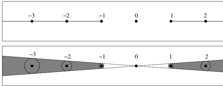
Fig. 4.1 Above, the domain \mathring{\mathcal{R}}^{(0)} . Below, the domain \mathring{\mathcal{R}}_\rho^{(0)} .
