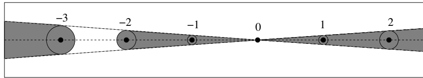
Fig. 4.6 The domain \mathring{\mathcal{D}}_\rho^{2,\pi} . The set \mathring{\mathcal{P}}_\rho^{(-)2,\pi} lies below the real axis, the set \mathring{\mathcal{P}}_\rho^{(+),2,\pi} lies above the real axis.
