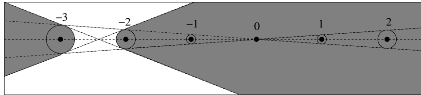
Fig. 4.5 The domain \dot{\mathcal{Q}}_\rho^{2,\pi} . The set \dot{\mathcal{Q}}_\rho^{(-)2,\pi} lies below the real axis, the domain \dot{\mathcal{Q}}_\rho^{(+ )2,\pi} lies above the real axis.
