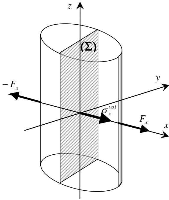
Figure 11 Schematic representation of a plane biaxial expansion of a cylinder. \sigma_x^{vol} is the normal stress applied on the section \Sigma .
