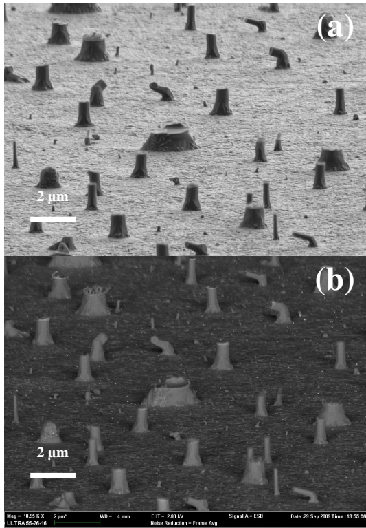
Figure 8 SEM images from Medium (M) wires after removing gold catalyst: (a) in secondary electrons mode and (b) in backscattered mode.
