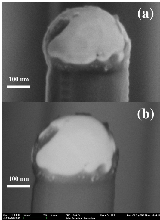
Figure 2 Details from SiNW head with several zones in the Au/Si alloy: (a) view in topographic mode, (b) view in chemical contrast mode, showing evidence of two parts in the alloy: rich and poor in Au.
