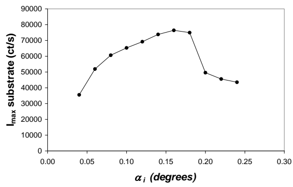
Figure 5 Absolute value of the intensity of the peak (Sub) versus the incidence angle \alpha_i .
