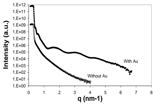
Figure 3 XRR profiles from SiNW samples with gold (dark circles) and without gold (open circles). The reflected intensity is plotted in arbitrary units versus the scattering vector q . The oscillations are evidence of the presence of gold particles.
