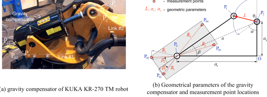
Fig. 2 Gravity compensator and its model
