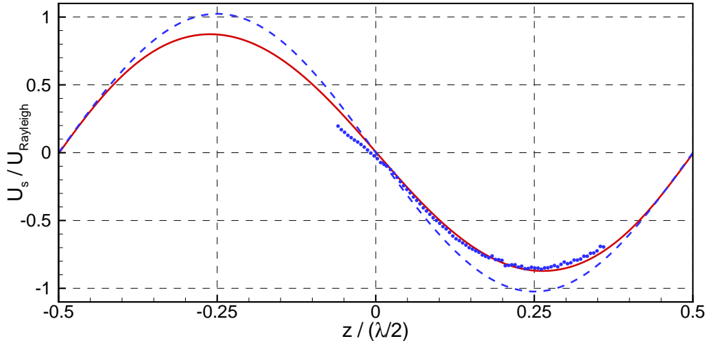
FIG. 5. (color online) Variation of the normalized axial streaming velocity component along the central axis of the guide. (—) Analytical results using the conditions of the experiment ; (●) E_2 , experimental measurements at Re_{NL} = 4.8 ; (—) N_2 , numerical simulation Re_{NL} = 4.91 .
