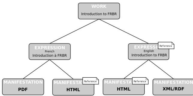
Figure 2: Document tree showing various translations and formats
