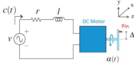
Figure 1: Sketch of the DC motor.
