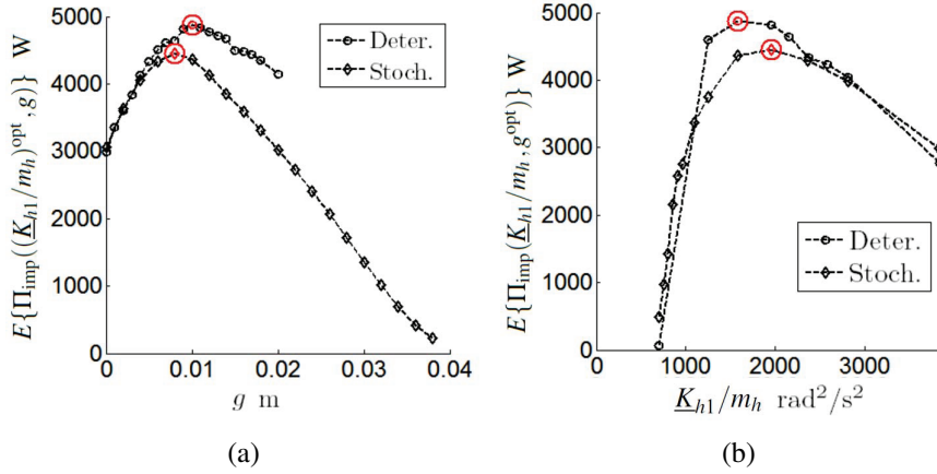
Figure 3: (a) Cost function as function of g with (\underline{K}_{h1}/m_h)^{\text{opt}} . (b) Cost function as function of \underline{K}_{h1}/m_h with g^{\text{opt}} . In both graphs, the E\{\Pi_{\text{imp}}(\mathbf{p}_{\text{des}}^{\text{opt}})\} is highlighted for the deterministic and stochastic cases with markers .
