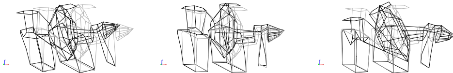
Figure 6: First 3 projected mode shapes for Pump 2.
