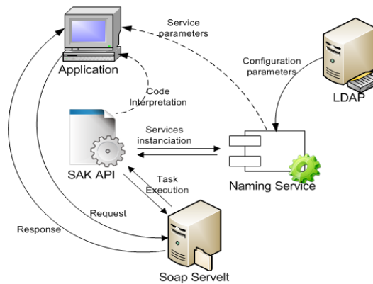
Figure 2. Internal and external interactions in the proposed framework
