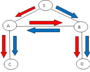
Figure 1: Initial tree T_0 (red) and final tree T_1 (blue)
