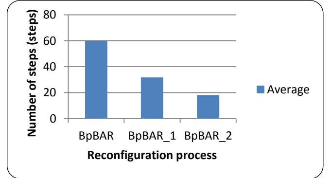
Figure 10: Average number of steps for each reconfiguration process in COST 239
