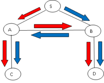
Figure 1: Initial tree T_0 (red) and final tree T_2 (blue)
