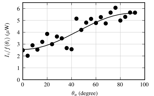
FIG. 11. Idler intensity I_i normalized over the polarisation response f(\theta_i) of the visualization setup and plotted as a function of the relative polarisation \theta_p of the pump and the probe. The dots are the experimental data. The probe polarisation is fixed vertically, while the pump polarisation is rotated incrementally between 0 degree (parallel) and 90 degrees (orthogonal). The solid curve is a fit including the effect of the two polarisation-dependent scattering channels.
