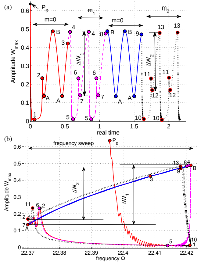
Fig. 13 Frequency sweep for Design 1: without added mass (solid line), with small mass m_1 = 10^{-5} (dashed line) and bigger mass m_2 = 10^{-4} (dotted line). (a): response W_{\max} - t ; (b): response W_{\max} - \Omega .
