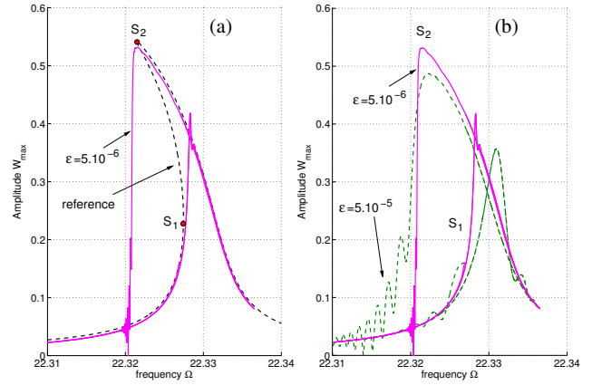
Fig. 18 Influence of \varepsilon on the response. (a) for \varepsilon = 5.10^{-6} (solid line) and reference response with ANM (dashed-dotted line); (b) \varepsilon = 5.10^{-6} (solid line) and \varepsilon = 5.10^{-5} (dashed line).
