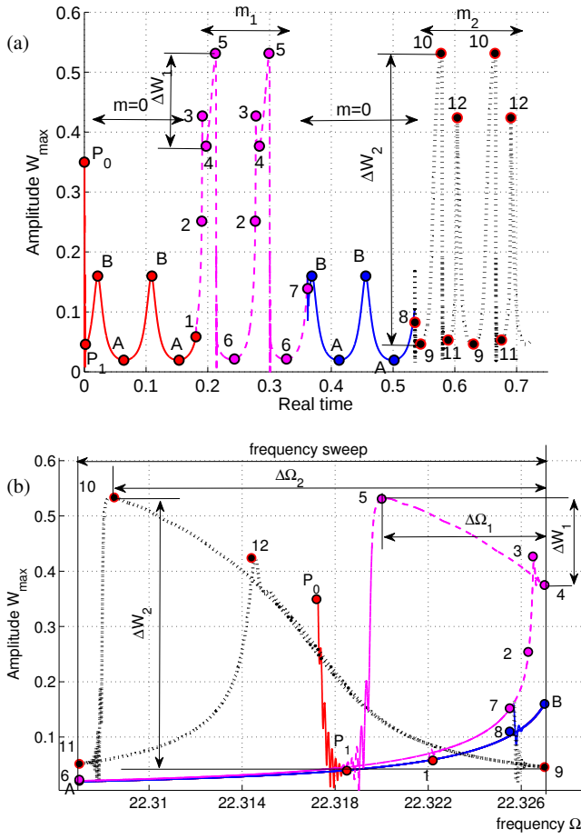
Fig. 10 Frequency sweep for Design 2. (a): response W_{\max} - t ; (b): response W_{\max} - \Omega . Without added mass (solid line); with small added mass (dashed line) and big added mass (dotted line).
