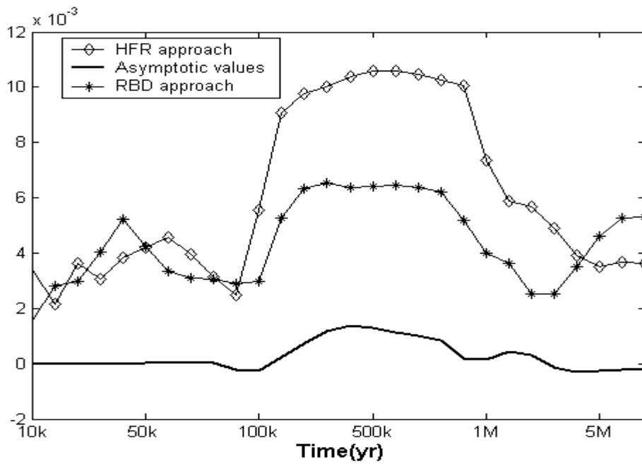
Figure 4 (c): Second Test Case: Level-E. Comparison between the RBD and the HFR approaches, for input factor 3.
