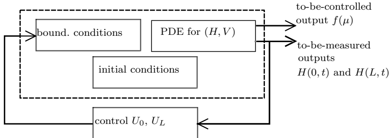
Fig. 2 Control loop in case when are no uncertainties.
