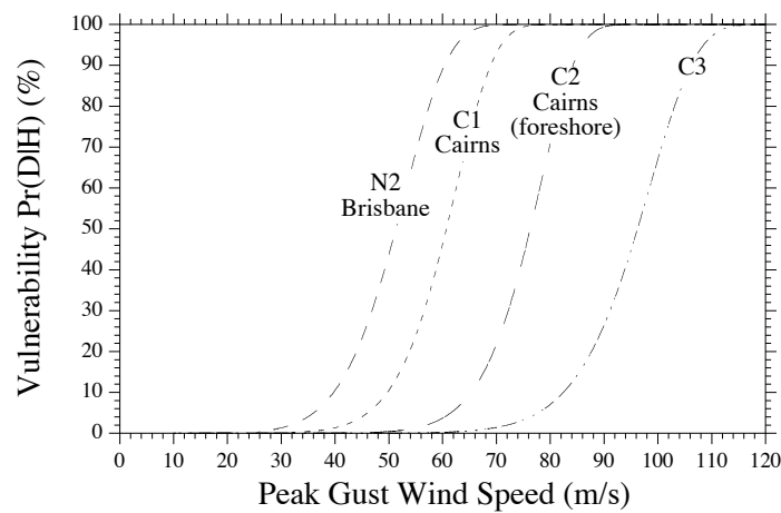
Figure 7: Wind vulnerability curves for residential construction in Queensland (adapted from Stewart et al. 2012b).
