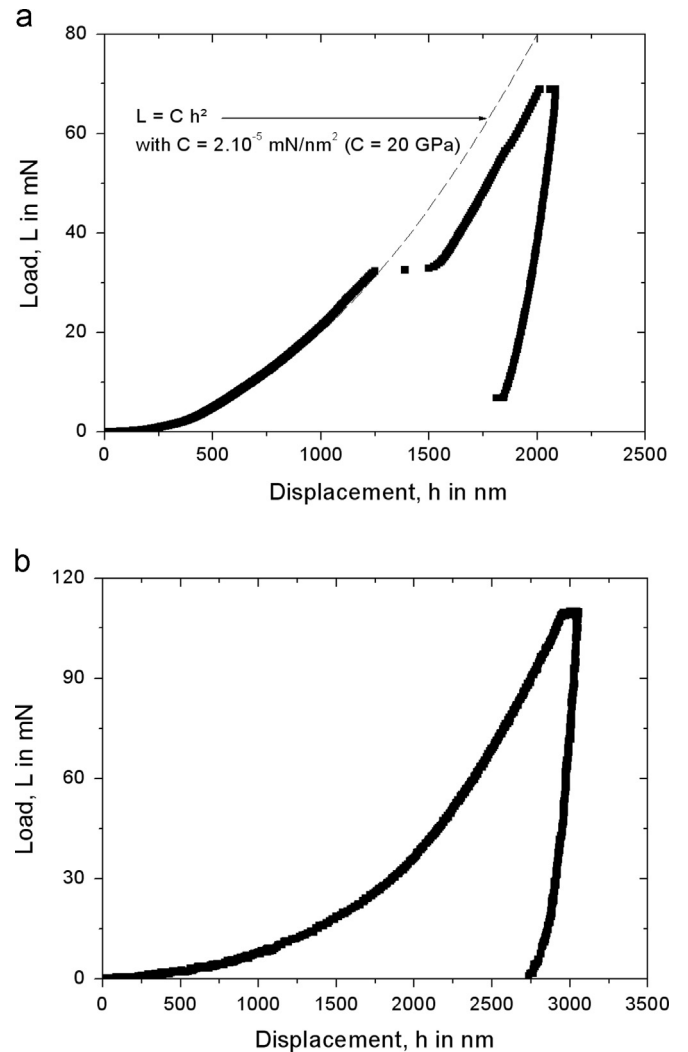
Fig. 3. Load–displacement curves obtained by CSM mode in nanoindentation (a) and by classical loading mode in microindentation (b).
