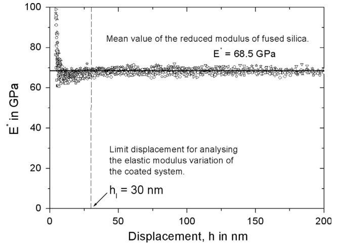
Fig. 7. Reduced modulus of fused silica for the contact area calibration of the Berkovich indenter used in nanoindentation.
