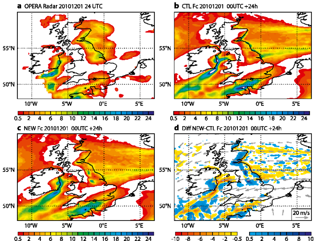
FIG. 11. 24-h precipitation accumulations (mm) for 1 Dec 2010 over the British Isles and near the European mainland from (a) radar observations on a 0.25° grid, and 24-h n = 1279 ( \Delta x = 16 km) forecasts with (b) CTL, (c) NEW, and (d) difference between NEW and CTL. The advection is represented in (d) by the mean 500–850-hPa wind. NEW improves the RMSE against observations by 2% compared to CTL.
