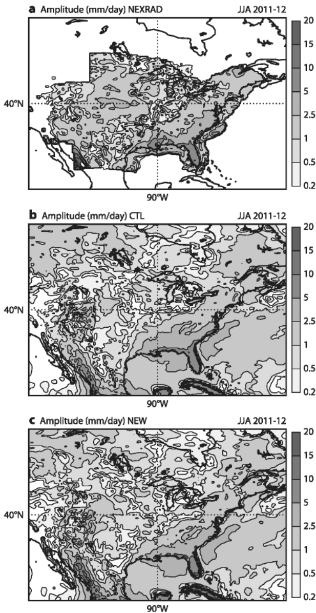
FIG. 3. Amplitude ( \text{mm day}^{-1} ) of the precipitation averaged over JJA 2011 and 2012 for the continental United States from (a) NEXRAD, and from daily 72-h forecasts at truncation n = 511 ( \Delta x = 40 km) with (b) CTL and (c) NEW closure. The RMSE against observations does not differ significantly between CTL and NEW.
