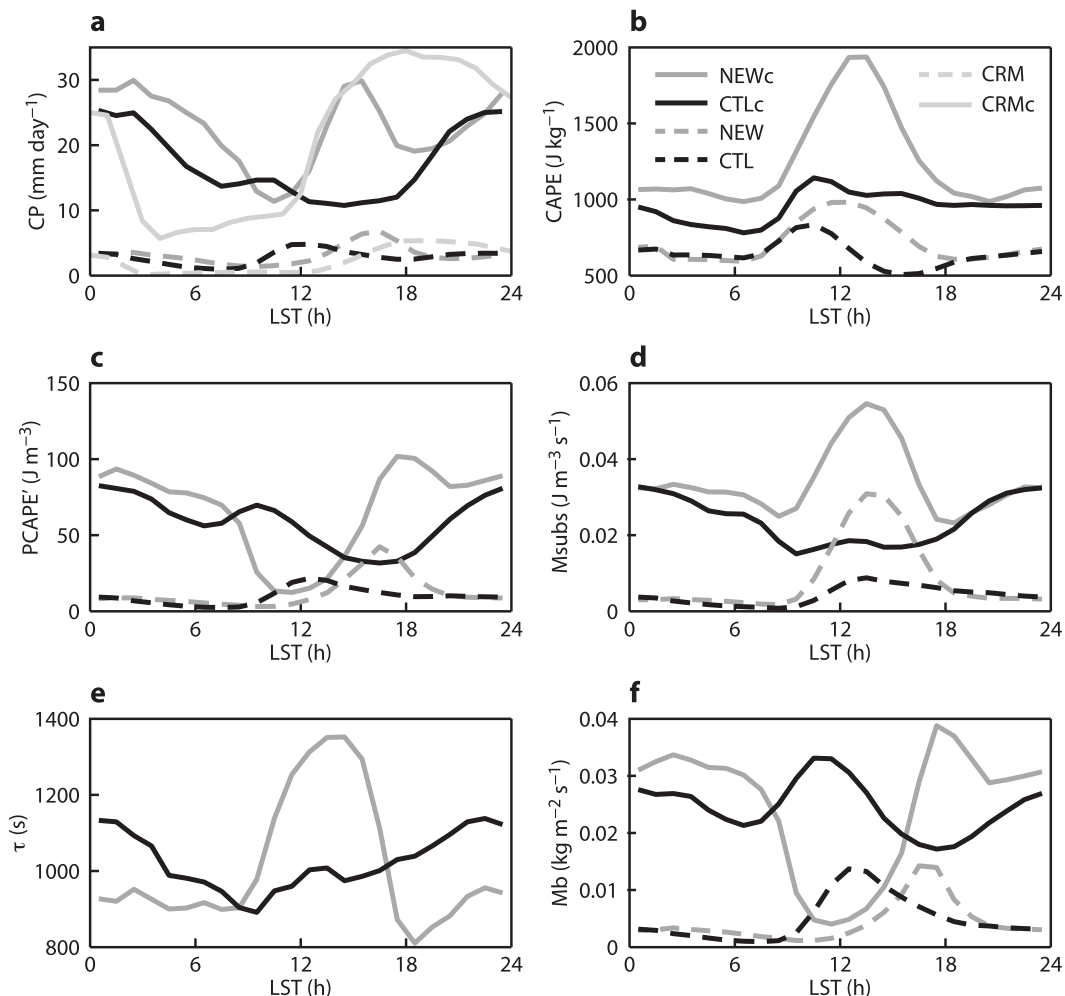
FIG. 6. Diurnal composites of convective closure-related diagnostics during 10–25 Jun 2012 over the central Sahel region: (a) Convective precipitation, (b) CAPE, (c) \text{PCAPE}' = \text{PCAPE} for CTL and \text{PCAPE} - \text{PCAPE}_{\text{BL}} for NEW, (d) the compensating mass flux term in (5), (e) the convective adjustment time scale, and (f) the cloud-base mass flux. Dashed lines denote total-area averages and solid lines and legends with suffix “c” denote averages over the regions with convective precipitation. Precipitation statistics from the CRM are included in (a), with the precipitation rates per rain event scaled to account for the difference in resolution between CRM and IFS.
