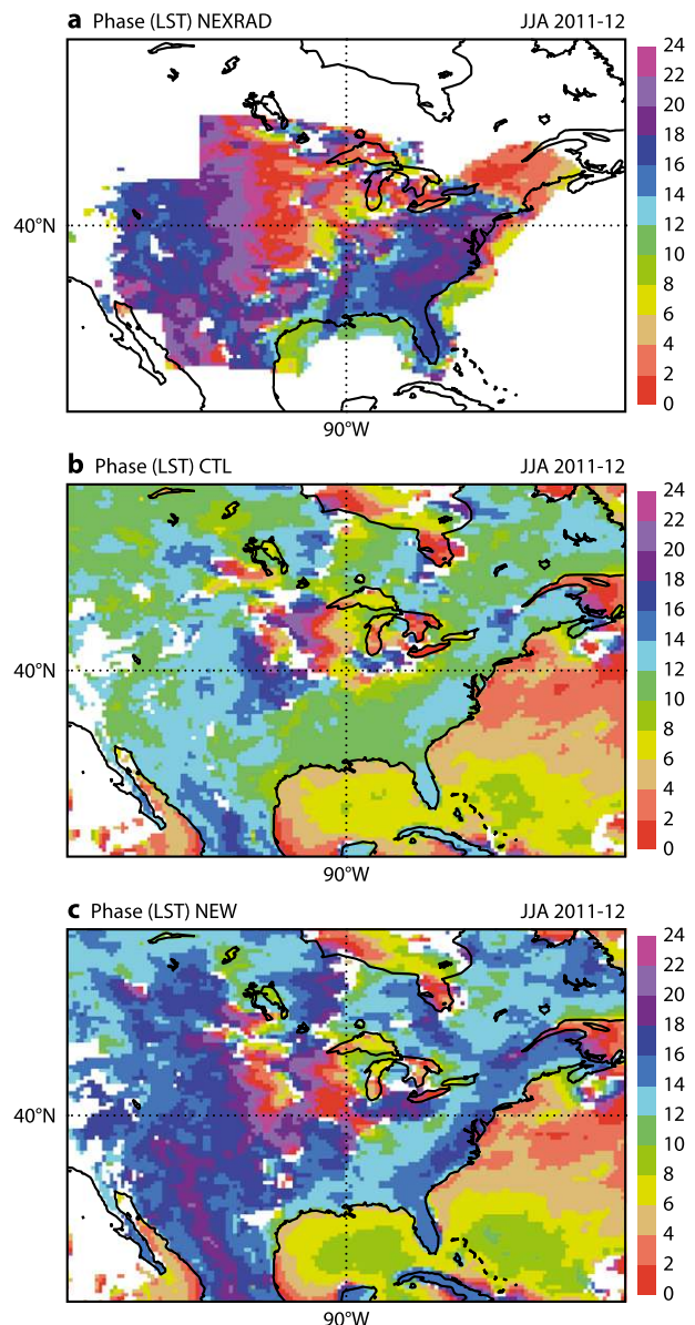
FIG. 4. As in Fig. 3, but for the diurnal phase of the precipitation (LST).
