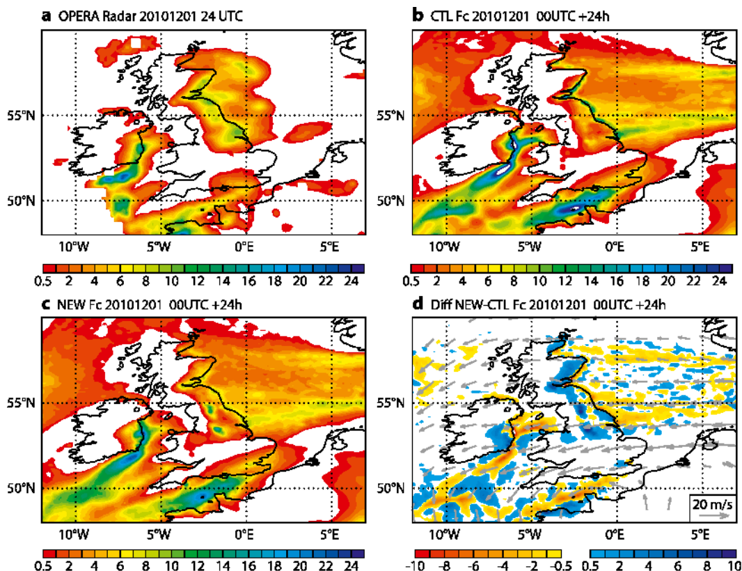
FIG. 11. 24-h precipitation accumulations (mm) for 1 Dec 2010 over the British Isles and near the European mainland from (a) radar observations on a 0.25^\circ grid, and 24-h n = 1279 ( \Delta x = 16\text{ km} ) forecasts with (b) CTL, (c) NEW, and (d) difference between NEW and CTL. The advection is represented in (d) by the mean 500–850-hPa wind. NEW improves the RMSE against observations by 2% compared to CTL.
