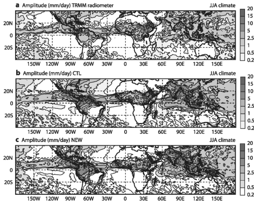
FIG. 1. Diurnal amplitude ( \text{mm day}^{-1} ) of the precipitation in the tropical band as obtained (a) from a 10-yr climatology of TRMM radiometer data (courtesy of Yukari Takayabu and colleagues), and from an ensemble of annual IFS integrations at truncation n = 159 ( \Delta x = 125 km) with (b) CTL and (c) NEW closure.
