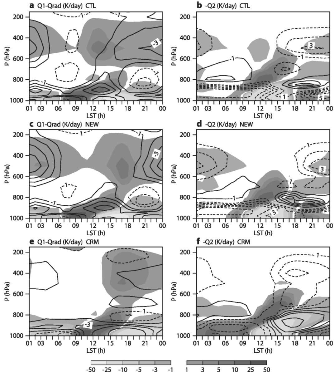
FIG. 7. Diurnal composites of heating and moistening rates ( \text{K day}^{-1} ) during 10–25 Jun 2012 over the central Sahel for (a),(b) CTL, (c),(d) NEW, and (e),(f) CRM. (left) Total heating rate minus radiation and (right) total moistening rate are shaded. Solid contour lines denote cooling and drying rates due to adiabatic motions; dashed contour lines (interval 1 \text{ K day}^{-1} ) denote adiabatic heating and moistening.
