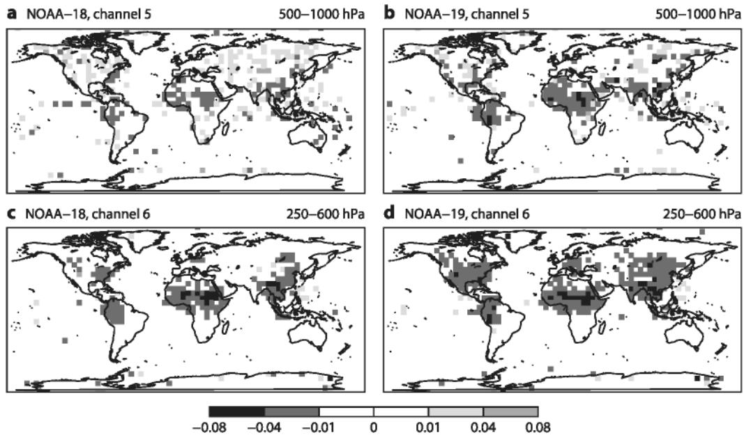
FIG. 9. Root-mean-square error differences in clear-sky BTs (K) for July 2012 between NEW and CTL during the 12-h window of the 4D-Var analysis, when evaluated against AMSU-A channels onboard NOAA sun-synchronous satellites. The channels are representative for different atmospheric layers: (a),(b) NOAA-18 and -19 channel 5 for the 500–1000-hPa layer, and (c),(d) NOAA-18 and -19 channel 6 for the 250–600-hPa layer. The twice-daily overpass times are 0300 and 1500 LST for NOAA-18 and 0130 and 1330 LST for NOAA-19 .
