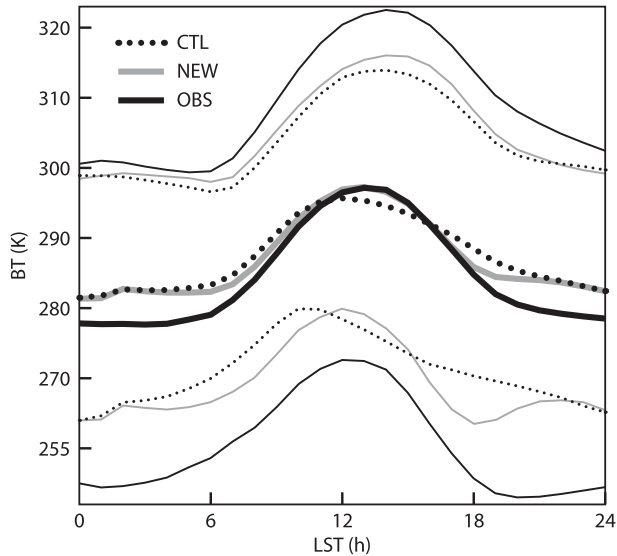
FIG. 8. Diurnal composite of mean and standard deviation of infrared BTs (K) in the 10.8\text{-}\mu\text{m} window during June–July 2012 over the central Sahel from Meteosat-9 , and from the day-2 CTL and NEW forecasts. The composites have been computed from a two-dimensional PDF, and a -3\text{-K} bias correction has been applied to the forecasts. Thick lines correspond to median values, and thin lines correspond to plus or minus one standard deviation.
