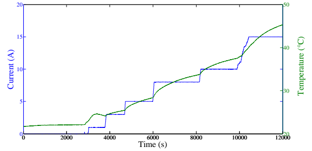
Figure 5. dynamic load profile and behaviour of the stack temperature
