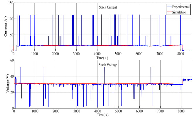
Figure 4. Stack voltage of FC
