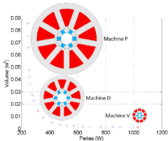
Figure 4. Front de Pareto volume - pertes
