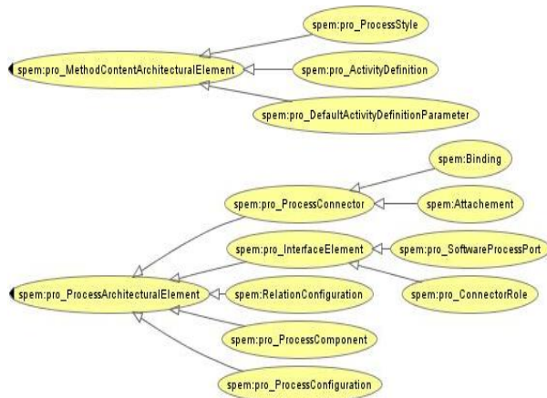
Figure 2: SP architectural concepts of SPEMontology.
