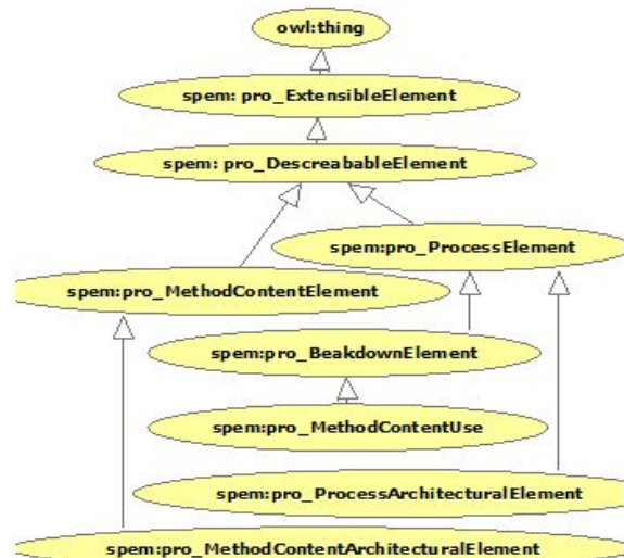
Figure 1: Main abstract SPEM Ontology concepts.
