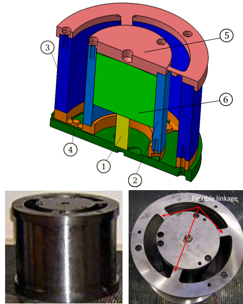
Fig. 8. Device integrating a PA
