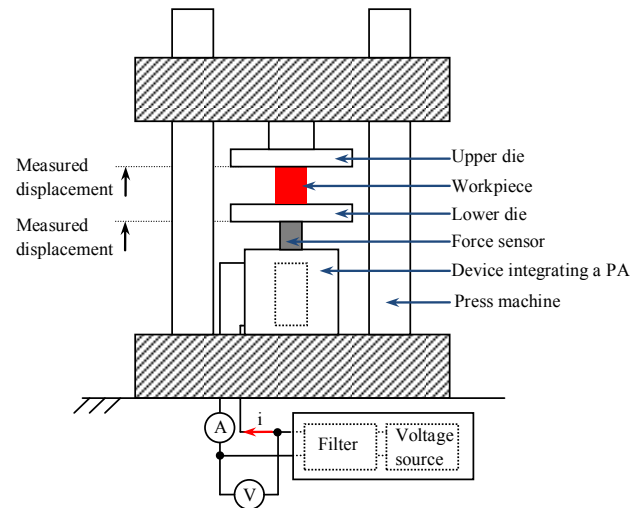
Fig. 2. Experimental setup
