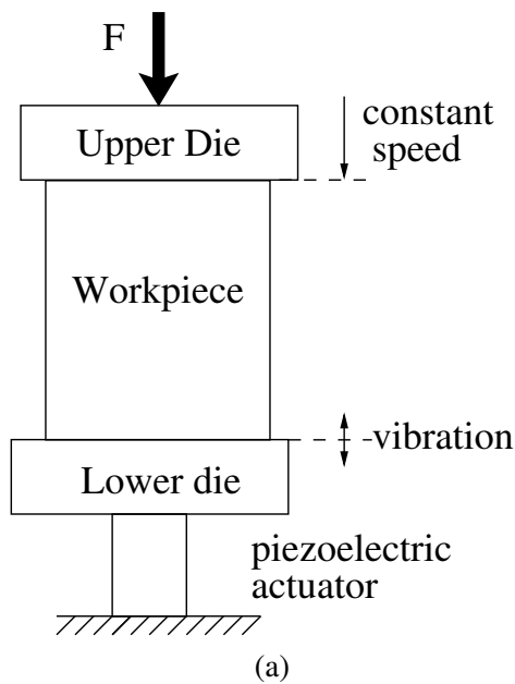
Figure 1: Vibrations assisted forging : (a) schematic of the process (b) Effects on the forging load
