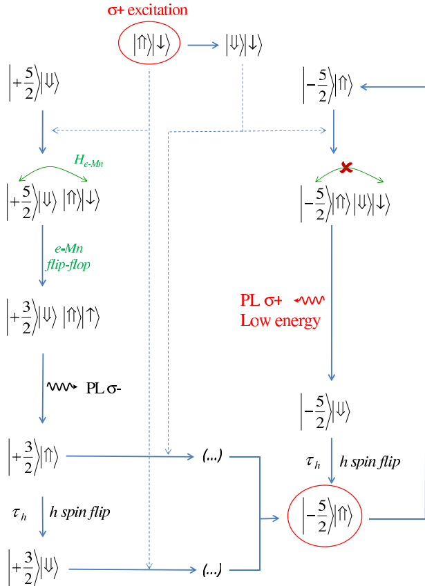
FIG. 3. (Color online) Scheme of the optical pumping mechanism of the spin of the hole-Mn complex under \sigma+ excitation. The electron-Mn flip-flops controlled by \mathcal{H}_{e-Mn} and the electron-Mn coherence time T_2^{eMn} prepare the Mn spin in the state S_z = -5/2 . See the text for a detailed description of the pumping process.
