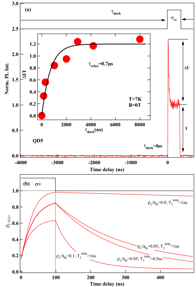
FIG. 7. (Color online) (a) Optical pumping transient obtained on the high-energy line of X^+ -Mn in QD5 under excitation with circularly polarized light trains of 300 ns separated by a dark time of \tau_{\text{dark}} = 8 \mu\text{s} (the excitation sequence is displayed on the top). Inset: Evolution of the amplitude of the optical pumping transient with \tau_{\text{dark}} for B = 0 \text{ T} and T = 7 \text{ K} . (b) Calculated time evolution in the dark of the population of the Mn spin state S_z = -5/2 initially pumped by a \sigma+ cw excitation (excitation sequence displayed at the top). The calculations are performed with the exchange couplings parameters of QD5 (see Table I), \tau_{Mn} = 5 \mu\text{s} , \tau_h = 1 \text{ ns} , \tau_r = 0.3 \text{ ns} , T_2^{eMn} = 0.1 \text{ ns} , T = 10 \text{ K} , a = 0.32 \mu\text{eV} , D_0 = 6 \mu\text{eV} , E = 0.5 \mu\text{eV} , and different amplitudes of valence-band mixing \rho_s/\Delta_{lh} and hole-Mn coherence time T_2^{hMn} .
