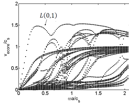
Fig. 3 Energy velocity of an embedded seven-wire strand.
