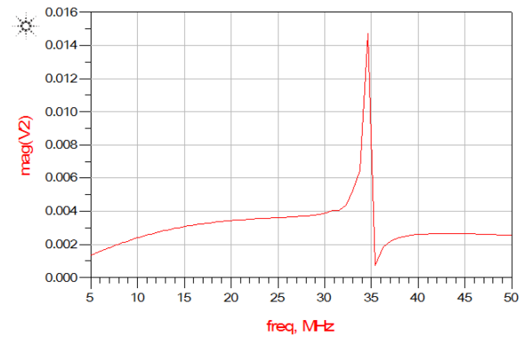
Figure 7- Voltage in the secondary with the metamaterial
