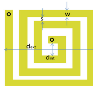
Figure 2- Unit cell of the prototype
