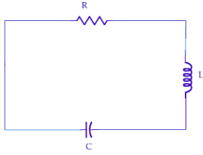
Figure 1- Model RLC of a coil in short circuit [15]
