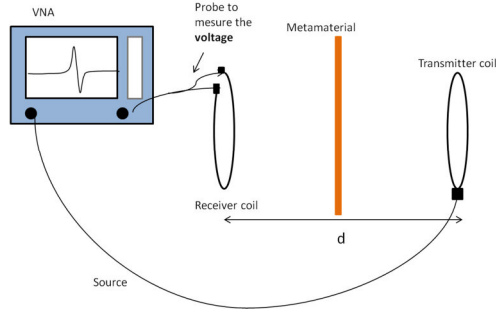
Figure 3- Experimental setup
