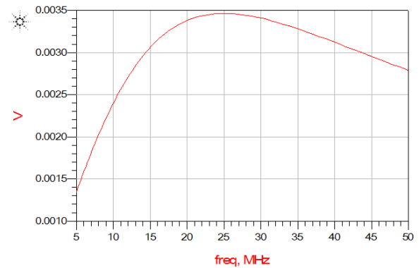
Figure 6- Voltage in the secondary without the metamaterial
