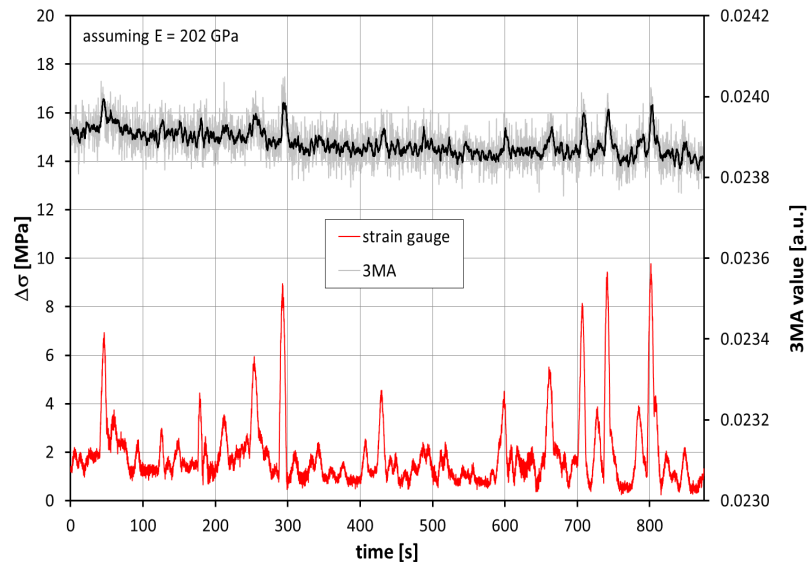
Figure 10. Strain gauge and micromagnetic signal of traffic load
