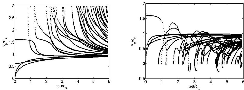
Figure 2. Calculated dispersion curve of guided wave modes in single z-shaped fiber (left: phase velocity; right: group velocity; a = 3 \text{ mm} , c_s = 3.2 \text{ mm}/\mu\text{s} )
