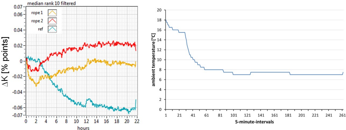
Figure 9. Change of harmonic distortion factor K (to the left, filtered by Median rank 10) and temperature (to the right) throughout the first experiment at the bridge
