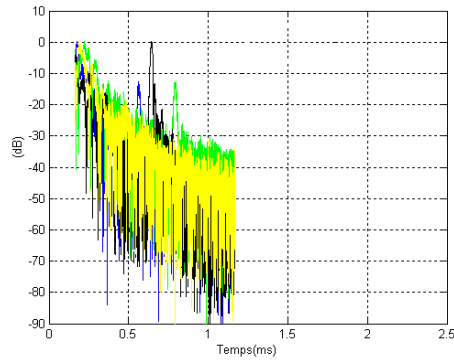
Figure 6. Time envelopes of echo signal for the damaged strand with 3 broken wires at 1.6 m case 1 (black curve), 2 m case 2 (green curve) and 1.4 m case 3 (blue curve). The yellow curve is for the central wire (undamaged wire).
