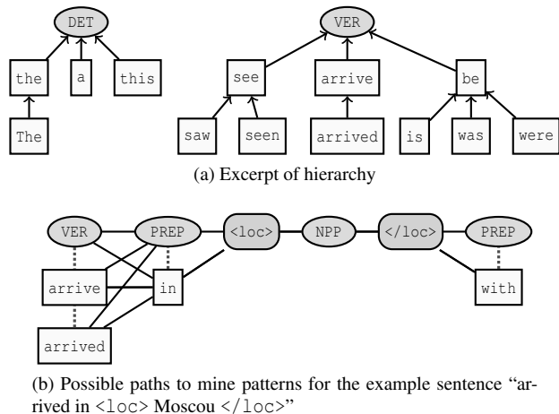
Figure 1: POS hierarchy and example of tagged sentence
