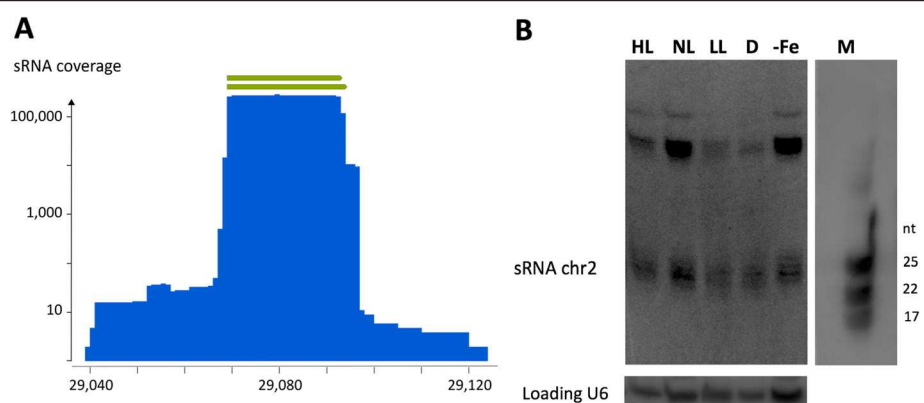
Figure 2 A novel sRNA population of unknown biogenesis from an intergenic region. (A) Screenshot of the reads profile of the mature small RNA populations matching an intergenic region in the chromosome 2 (chr2: 29.039-29.123), with reads belonging to the five small RNA libraries. (B) Validation of the sRNAs expression by low molecular weight Northern blotting. Total RNA was extracted from cell cultures grown under different light conditions (High Light (HL), Normal Light (NL), Low Light (LL), Dark (D) and iron starvation (-Fe)) and Northern blots hybridized with radiolabeled probes recognizing the small 25 nt product and the U6 snRNA as reference loading control. M, microRNA Marker (New England Biolabs, USA).
