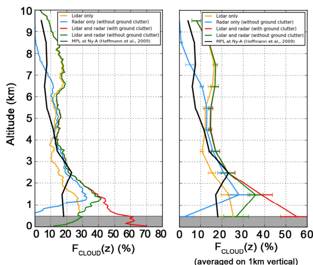
Figure 2. Vertical profiles of cloud occurrences over the Ny-Ålesund station during March and April 2007. The black line refers to ground-based lidar observations at 1 km vertical resolution (Hoffmann et al., 2009) and the coloured lines refer to a DARDAR product, according to different configurations and settings. DARDAR retrievals have a vertical resolution of 60 m on the left panel and 1 km on the right panel.
