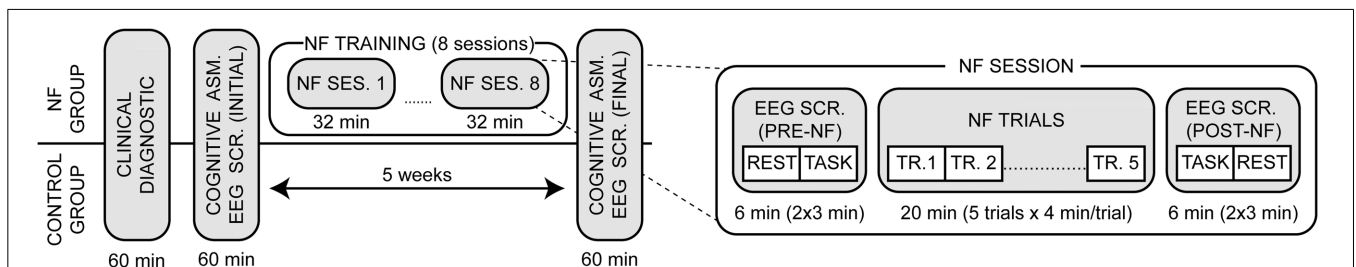
FIGURE 1 | Experimental design of the study. After an intake diagnostic both groups executed a pre- and post- cognitive assessment and EEG screening within a 5-week time interval. The NF group performed a total of eight NF
