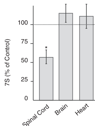
Figure 9. Analysis of endogenous 7S RNA level in tissues of SMA mice. Total RNA from the spinal cord, brain and heart of post-natal Day 10 control and SMA mice were analyzed by real-time RT-PCR. The level of 7S RNA was monitored by five independent biological replicates ( n = 5 ). The relative amount of 7S RNA in SMA mice tissues is plotted as percent of the controls. RPS29 mRNA was used to normalize the RNA input. The level of 7S RNA in spinal cord was significantly reduced in SMA mice, whereas its levels in brain and heart remain the same ( P < 0.05 ).
