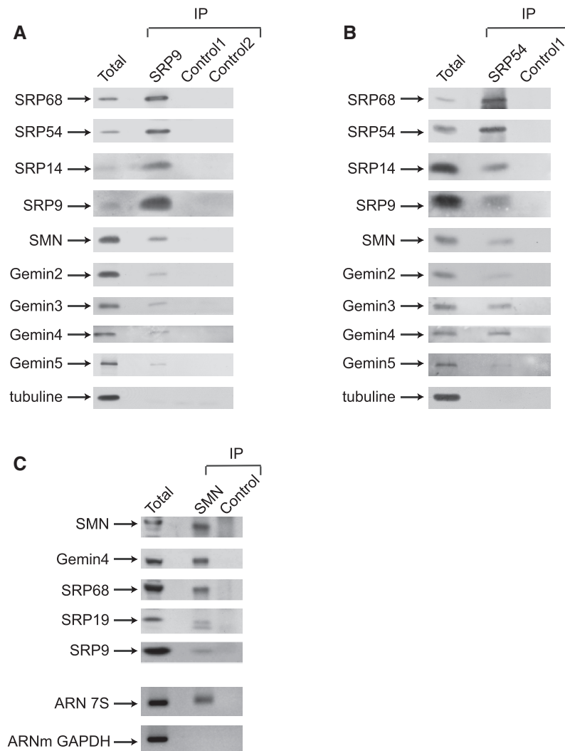
Figure 6. The SMN complex associates with SRP in HeLa cell extracts. IP experiments were carried out on HeLa cytoplasmic extracts using anti-SRP9 (A), anti-SRP54 (B), or anti-SMN 4B3 (C) antibodies bound to A-sepharose [in (A) and (B)] or G-dynabeads [in (C)]. The unrelated anti-Sox2 and anti-Lin28 antibodies were used as negative controls in (A) (Controls 1 and 2, respectively). A-sepharose alone was used as control in (B) and negative control mouse IgG (DAKO) in (C). The immunoprecipitated proteins were analyzed by SDS-PAGE and western-blotting with antibodies to the indicated proteins; 3% of the inputs are shown (Total). The immunoprecipitated RNAs were analyzed by RT-PCR in (C).
