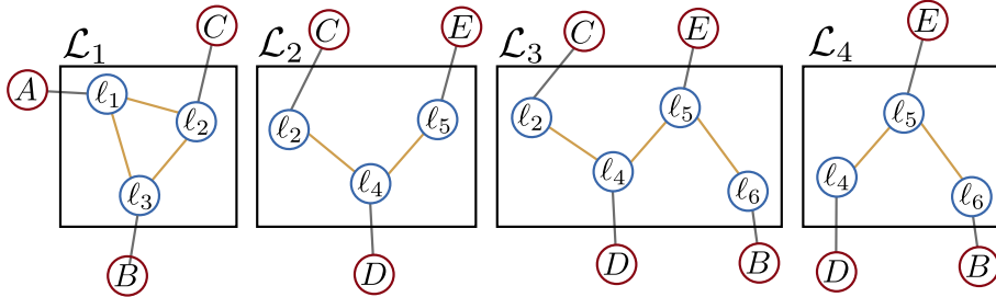
Figure 3: Given the query \mathcal{Z}_q = \{C, D, E\} and covisibility map \mathcal{M}_k (both shown in Fig. 2), will produce four virtual locations, \mathcal{L}_1, \mathcal{L}_2, \mathcal{L}_3 & \mathcal{L}_4 .
