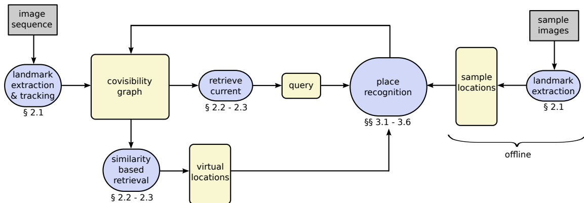
Figure 9: General scheme of the framework, with inputs depicted by rectangles, data structures depicted by rounded boxes, and algorithmic blocks depicted by ovals. Relevant section numbers for each algorithm are also shown for reference.
