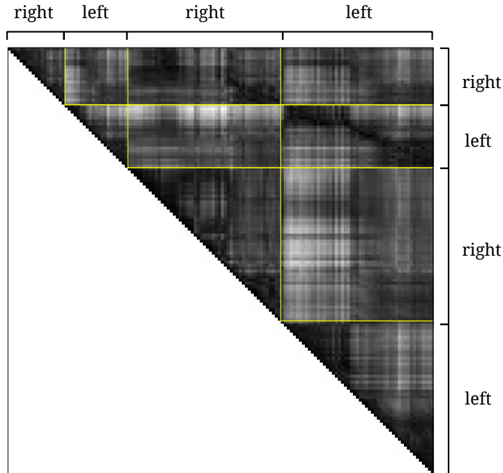
Figure 20: The confusion matrix when comparing differences (SAD) between all the images of the street sequence, with lighter pixels indicating larger differences. Highlighted lines indicate the start of each new traverse down the street. Only half the matrix is shown because of symmetry. The SeqSLAM algorithm [Milford, 2013] searches for diagonals of low difference values in the matrix.
