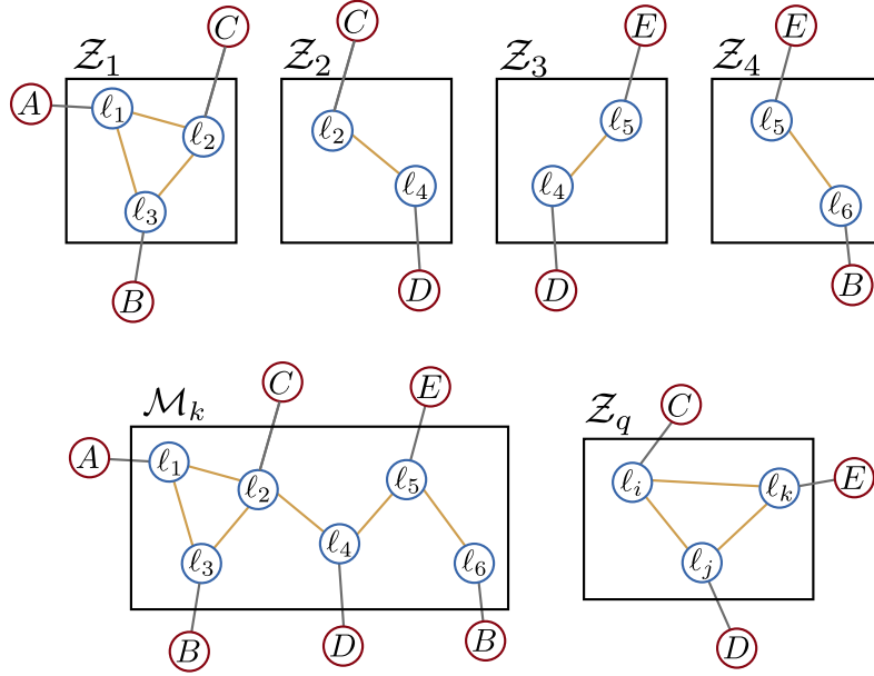
Figure 2: A sequence of simplified example observations is shown in the top row ( \mathcal{Z}_1, \mathcal{Z}_2, \mathcal{Z}_3, \mathcal{Z}_4 ), along with the corresponding covisibility map, \mathcal{M}_k , on the bottom-left, and the current query observation, \mathcal{Z}_q , on the bottom-right. The figure also depicts which word (represented as A, B, C, D or E ) is associated with each landmark, l_i .
