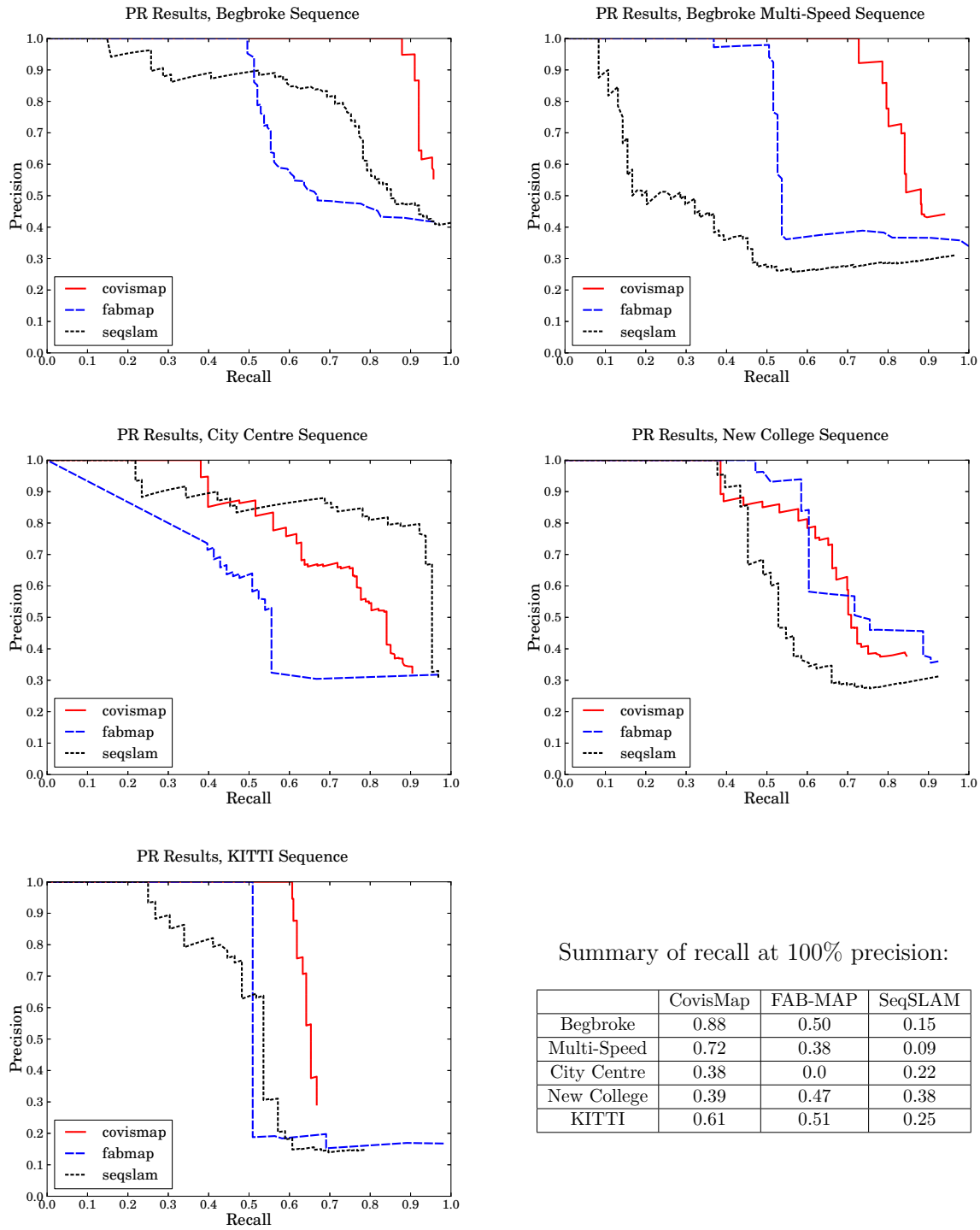
Figure 10: Precision-recall results for three methods (CovisMap, FAB-MAP, and SeqSLAM), tested on the Begbroke, Begbroke Multi-Speed, CityCentre, New College, and KITTI datasets.
