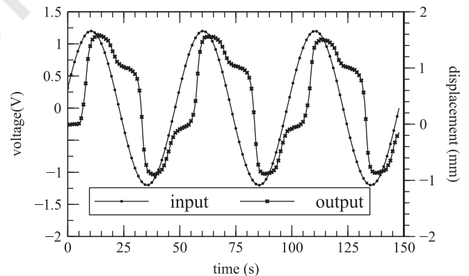
Fig. 11. Output of the controlled SMA actuator for the 2nd order filters ( H_p=3, r=0 ) with forgetting factor equal to 0.99.
