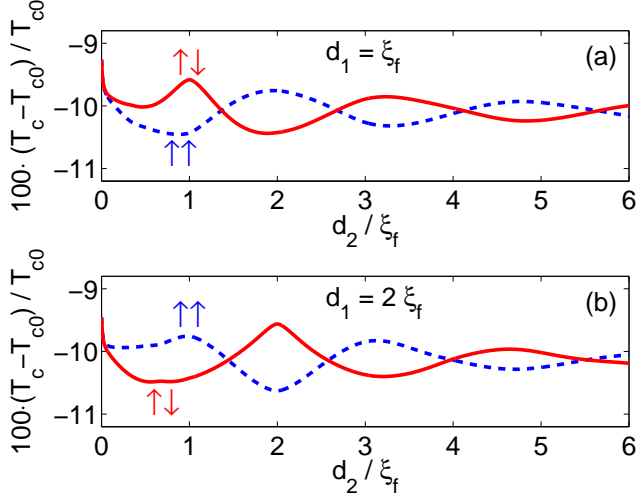
FIG. 2: (Color online) The dependencies of the critical temperature of the clean F_1/S/F_2 spin valve for parallel (blue dashed curves marked \uparrow\uparrow ) and anti-parallel (red solid curves marked \uparrow\downarrow ) orientations of magnetic moments on the width d_2 of the F_2 ferromagnetic layer. The width of the F_1 layer takes the values (a) d_1 = \xi_f and (b) d_1 = 2\xi_f (here \xi_f = v_f/4\pi T_{c0} ). Other parameters are h_1 = h_2 = 2\pi T_{c0} , 4\pi T_{c0}d_s/v_s = 0.1 and p_f = 0.2p_s .
