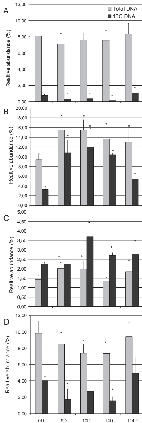
Figure 3: Relative abundances of phylum-specific 16S rRNA genes in soil DNA during incubation with 13 C-phenanthrene. Template was either total soil DNA (grey bars) or 13 C-DNA (black bars) extracted from SIP2000 experiments at 5, 10 and 14 days (5D, 10D and 14D, respectively). A control DNA sample was obtained from soil incubated for 14 days
