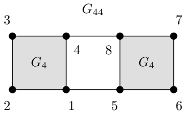
(c) The graph G_{44} .
