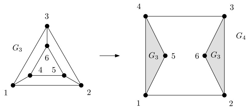
(b) The graphs G_3 (left) and G_4 (right).
