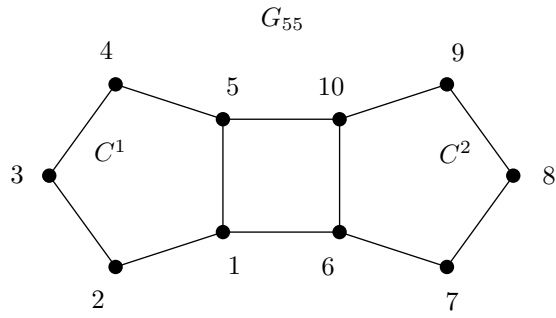
(a) The graph G_{55} .
