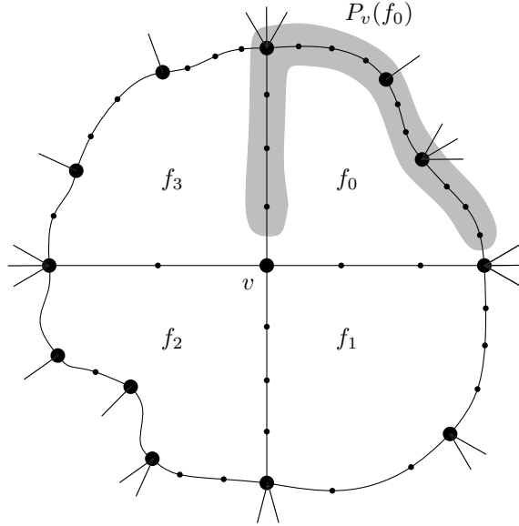
Figure 2.2. The definition of the path P_v(f_i) for i = 0 and a vertex v of degree 4. High-degree vertices are shown as larger dots.
