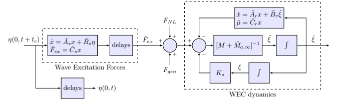
Fig. 8. Block diagram representation for state-space approximated Cummins model.
