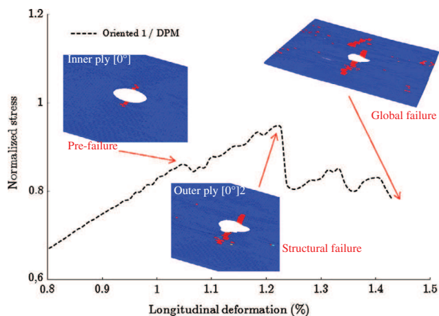
Fig. 16. Fibre failure at structural failure and global failure of Oriented 1 layup.
