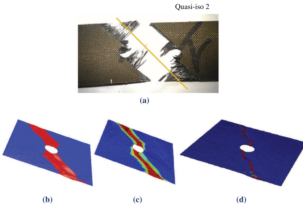
Fig. 8. Comparison of failure pattern at UTS for quasi-iso 2 layout [0/45/90/-45] 2s (a) bottom view, (b) matrix cracking, (c) delamination in 0^\circ/45^\circ interface, and (d) fibre failure in outer 0^\circ ply.
