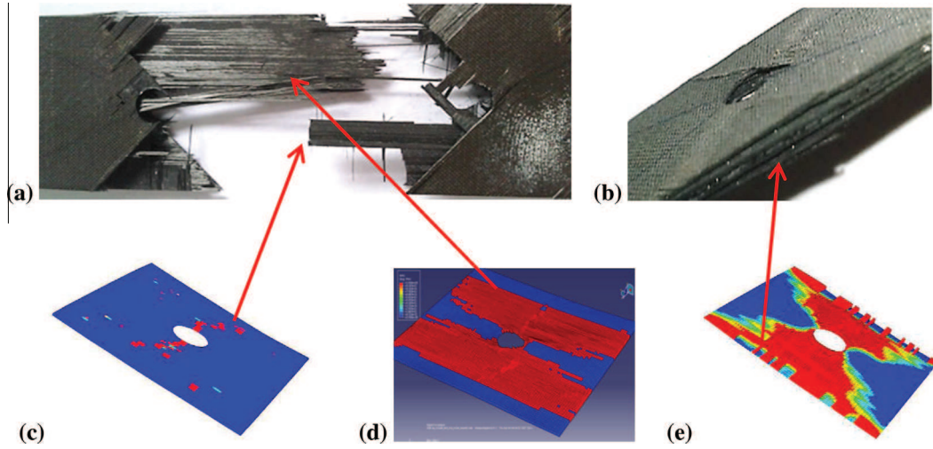
Fig. 9. Comparison of failure pattern at UTS for Oriented 2 layup [45/-45/0/0/90/0/0/-45/45] (a) bottom view, (b) side view, (c) fibre failure in [0_2] plies, (d) matrix cracking in [0_2] plies, and (e) delamination at [0/90] interface.
