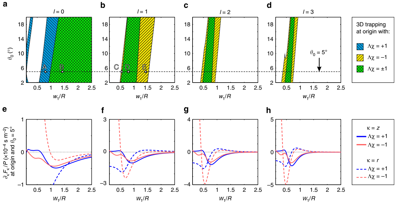
Figure 3 | Helicity-dependent 3D optical trapping simulations. (a-d) Existence of 3D trapping in the plane of parameters ( w_1/R , \theta_0 ) depending on the photon helicity for w_1 = 20 \mu\text{m} and l = 0, 1, 2 and 3 , where the material parameter values are those of our experiments. Three different coloured/hatched regions refer to trapping existence for the cases \Lambda\chi = +1 alone, \Lambda\chi = -1 alone and \Lambda\chi = \pm 1 simultaneously. Letters A, B, C, D and E correspond to the values w_1/R \approx 0.8, 1.43, 0.59, 0.74 and 1.43 . (e-h) Partial derivatives of the optical force components at origin per unit power for a beam divergence angle \theta_0 = 5^\circ .
