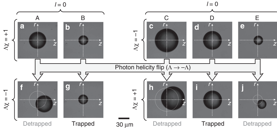
Figure 4 | Helicity-dependent 3D optical trapping observations. (a-e) Snapshots of onion-like chiral liquid crystal droplets optically trapped at origin under power P \approx 50 mW in situations tagged by the letters A, B, C, D and E in Fig. 3a-e, which, respectively, correspond to w_1/R \approx 0.8, 1.43, 0.59, 0.74 and 1.43 . Situations A and B refer to Gaussian beams with \Lambda\chi = +1 (a,b), whereas C, D and E refer to first-order Laguerre-Gaussian beams with \Lambda\chi = -1 (c-e). For l = 0 , helicity flip leads to detraping of the larger droplet (f), whereas the smaller one is kept trapped at the origin (g). For l = 1 , helicity flip leads to detraping for both the larger and the smaller droplets (h,j), whereas the droplet with intermediate size remains trapped at the origin (i).
