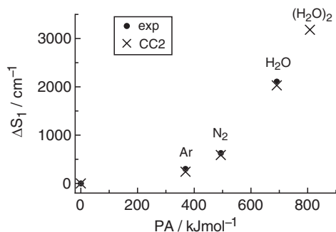
FIG. 7. Experimental and calculated \Delta S_1 shifts of \text{cis-BZH}^+ \cdot \text{L}_n as a function of the proton affinity of \text{L}_n . Calculated values are obtained at the ri-CC2/aug-cc-pVDZ level (Table IV).
