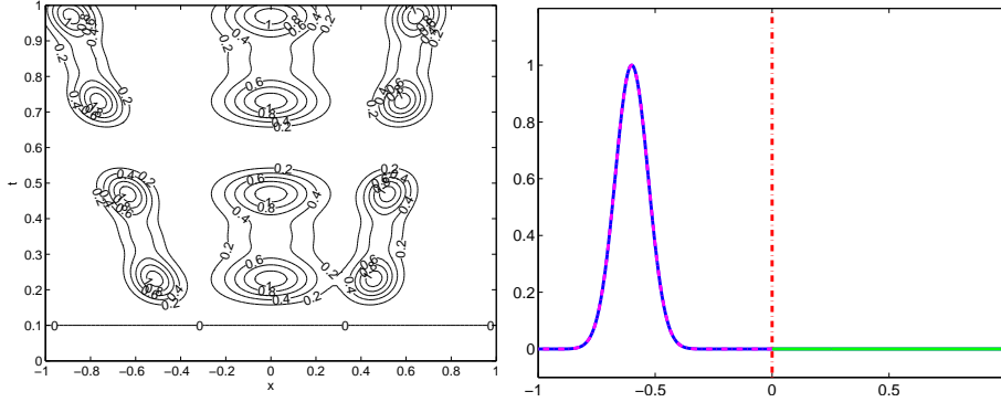
FIG. 5.1. Left: contour plot for the right hand side in space and time. Right: initial condition a > 0
