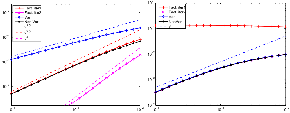
FIG. 5.3. Errors for a > 0 as the viscosity becomes small for our factorization algorithm compared to other coupling algorithms from the literature. Left: \|u - u_{ad}\|_{L^2_{x,t}} . Right: \|u - u_a\|_{L^2_{x,t}} .
