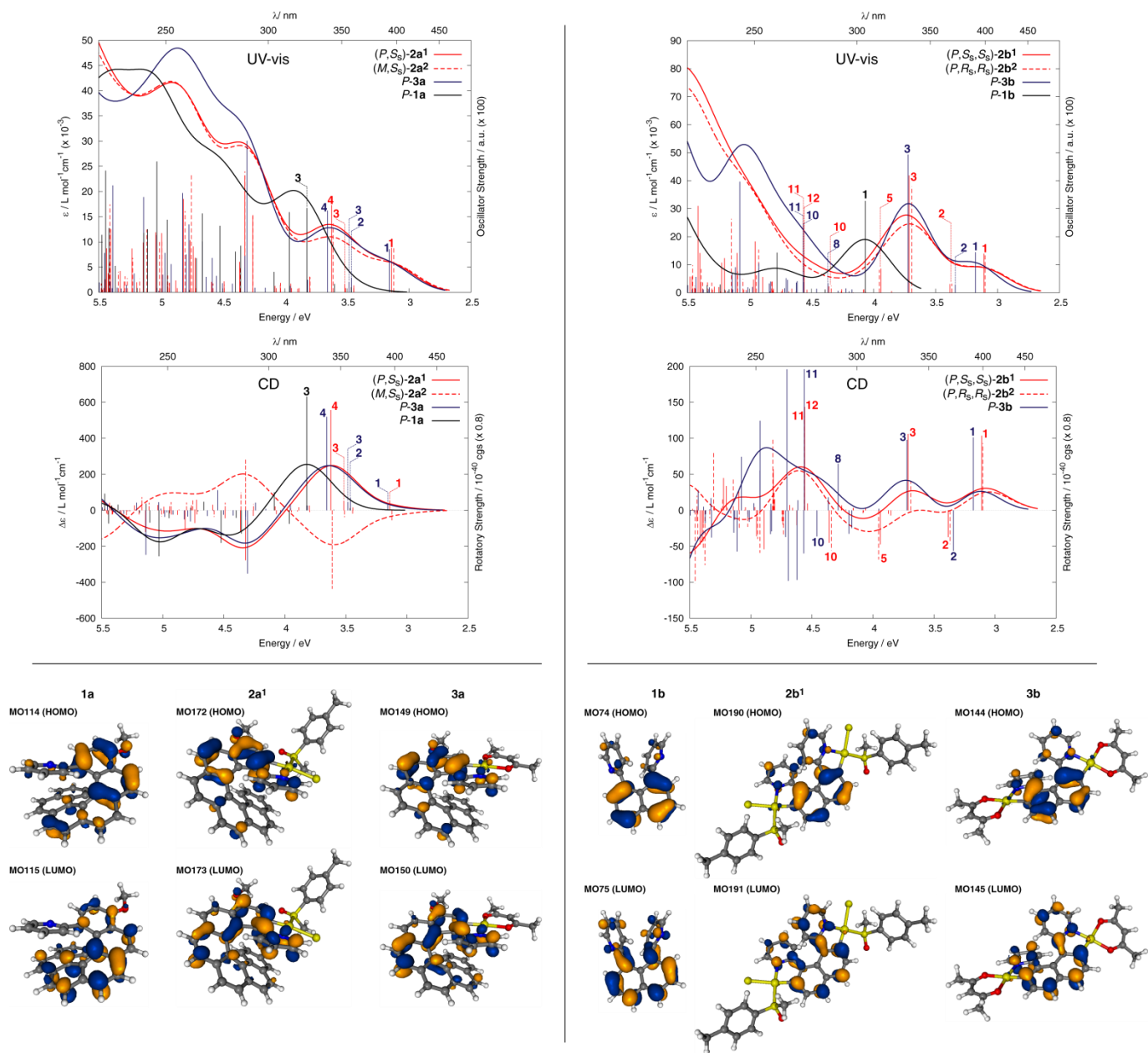
Figure 4. Comparison of the calculated UV-vis (top) and CD spectra (bottom) of P - 1a , P - 3a , ( P,S S )- 2a 1 and ( M,S S )- 2a 2 (left) and P - 1b , P - 3b , ( P,S S ,S S )- 2b 1 and ( P,R S ,R S )- 2b 2 systems (right). Color and line schemes correspond to those in Figure 3. No spectral shifts were applied. Numbers correspond to excitations that were analyzed in detail. Below isosurface plots of the HOMO and LUMO of series 1a , 2a 1 , and 3a and of series 1b , 2b 1 , and 3b are shown. Further details are provided in the ESI.
