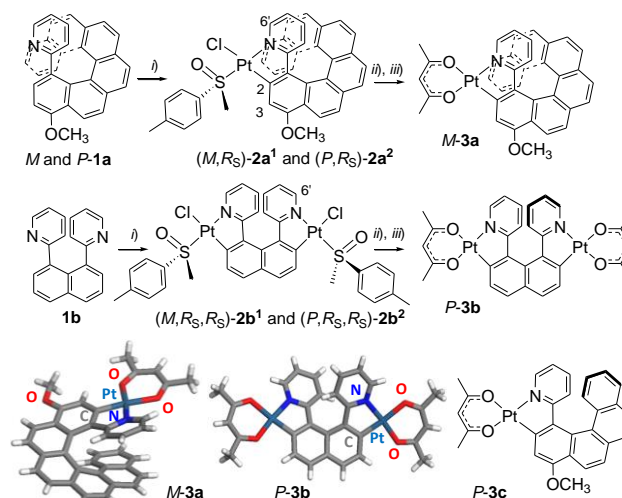
Scheme 1. General synthesis of enantiopure Pt[8]helicene and Pt 2 [6]helicene derivatives M-3a and P-3b from ( \pm )- 1a and 1b respectively. i ) ( S_5,S_5 )-PtCl 2 ( p -tolyl-MeSO) 2 , toluene, Na 2 CO 3 , Ar, reflux, overnight, 60%; ii ) column chromatography and/or crystallization; iii ) pentane-2,4-dione, toluene, Na 2 CO 3 , Ar, reflux, 2 h. X-ray crystallographic structures of 3a and 3b (one enantiomer shown) and chemical structure of 3c . 4a,b
