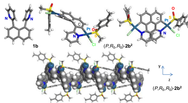
Figure 2. X-ray crystallographic structures of ligand 1b and the pure diastereomeric complex ( P,R S ,R S )- 2b 1 . Columnar packing of ( P,R S ,R S )- 2b 1 is observed along the z axis (Pt 2 -[6]helicene shown in CPK model representation).
