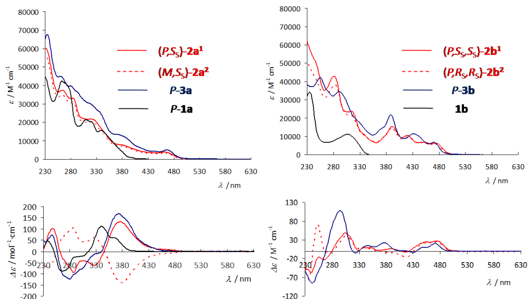
Figure 3. UV-vis and CD spectra of (P,S_5)\text{-}2\mathbf{a}^1 , (M,S_5)\text{-}2\mathbf{a}^2 , P\text{-}3\mathbf{a} , (P,S_5,S_5)\text{-}2\mathbf{b}^1 , (P,R_5,R_5)\text{-}2\mathbf{b}^2 , and P\text{-}3\mathbf{b} in solution in dichloromethane at room temperature, compared to the starting organic ligands P\text{-}1\mathbf{a} and \mathbf{1b} .
