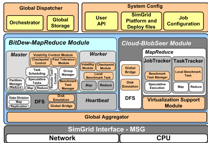
Fig. 3. BIGhybrid Simulator Architecture
