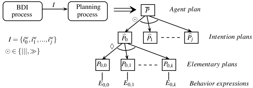
Fig. 1 Agent cycle
