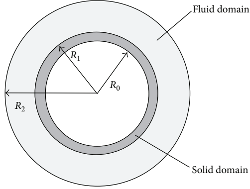
FIGURE 3: Geometry of fluid-solid interaction model. R_0 and R_1 are the inner and outer radius of solid domain, respectively.
