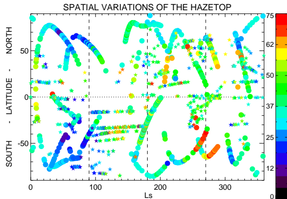
Figure 1: The whole hazetop dataset as a function of latitude and season. The circles and stars represent solar and stellar occultations, respectively. The color scale gives the hazetop altitude.
