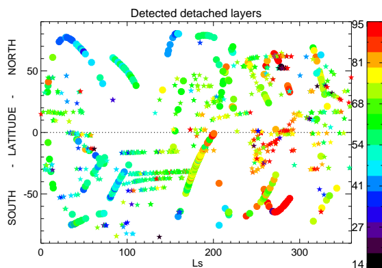
Figure 2: The detached layer dataset as a function of latitude and season. The circles and stars represent solar and stellar occultations, respectively. The color scale gives the detached layer altitude.
