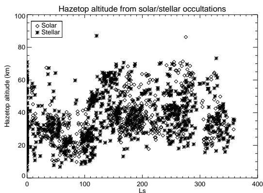
Figure 3: The hazetop altitude as a function of season.
