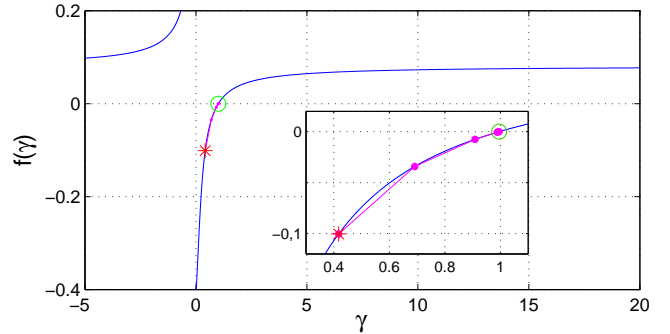
Figure 15. Example of function f(\gamma) (see equation (31)) whose zero is sought for using the Newton-Raphson method. In this example, the solution is \gamma^* = 1 . The initialisation point (red star) located at the left of the desired root (green circle) ensures the fast convergence of the method. The subfigure emphasises this convergence through the progress of the first three iterations (purple points).
