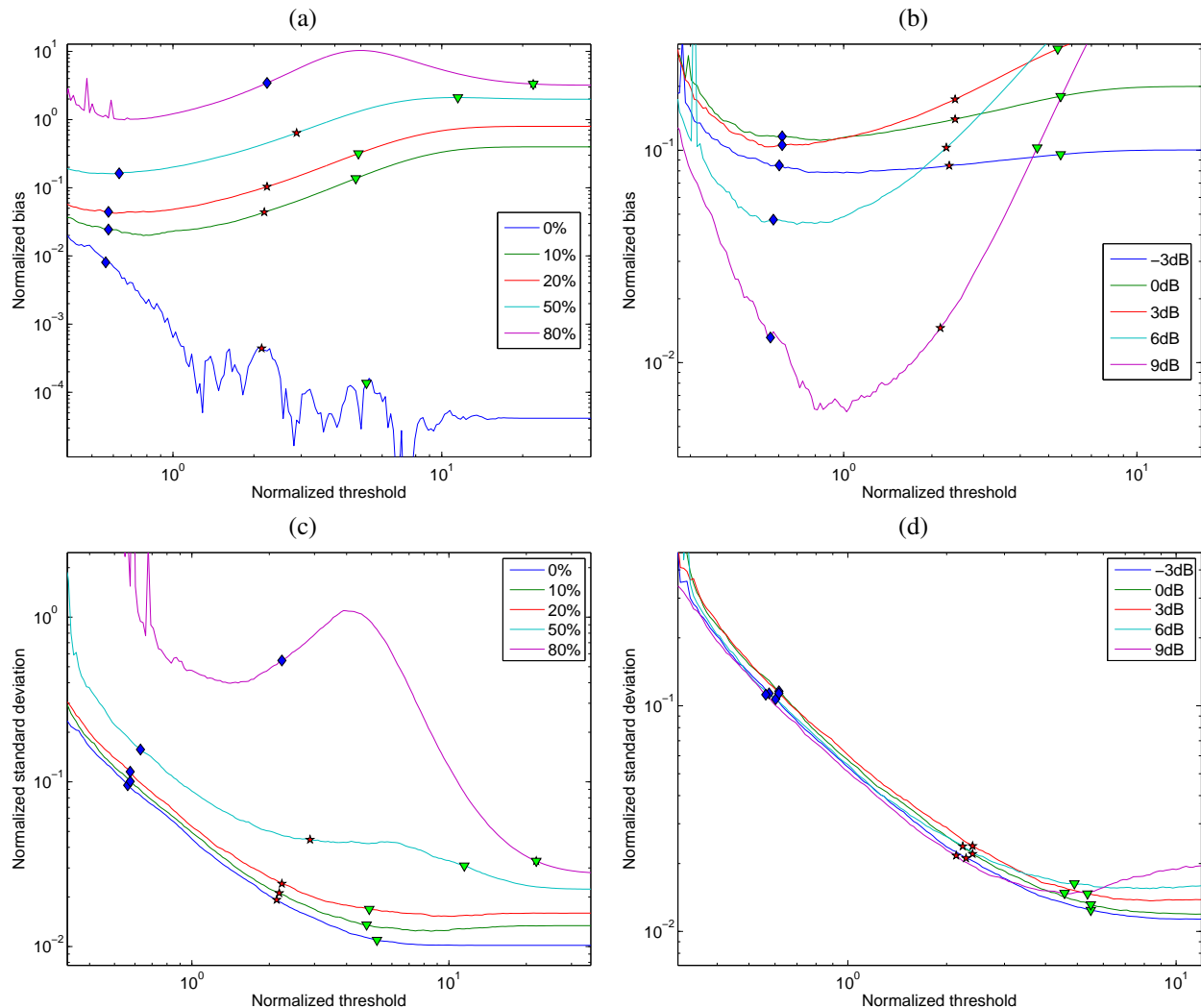
Figure 3. Performances of the MiniSMaL noise estimator in presence of a deterministic signal. Left column: (a) absolute value of the normalized bias and (c) normalized standard deviation for SNR = 4\text{dB} and for different signal proportion P . Right column: (b) absolute value of the normalized bias and (d) normalized standard deviation for a signal proportion P = 20\% and for different SNR. The results are obtained over 2000 noise runs. For each plot, the markers identify the operating points obtained with a spectral kurtosis \kappa equal to -0.6 (Blue diamonds), -0.4 (red stars) and -0.1 (green triangles). These latter points are described in section V.
