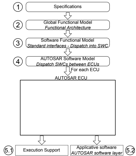
Figure 3: Automotive embedded software Process
