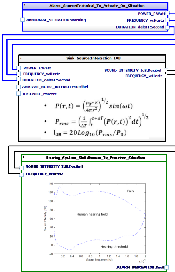
Fig.7: Specification S_{EE} of audible alarm (Source) perception by a human (Sink) represented in SysML IBD
